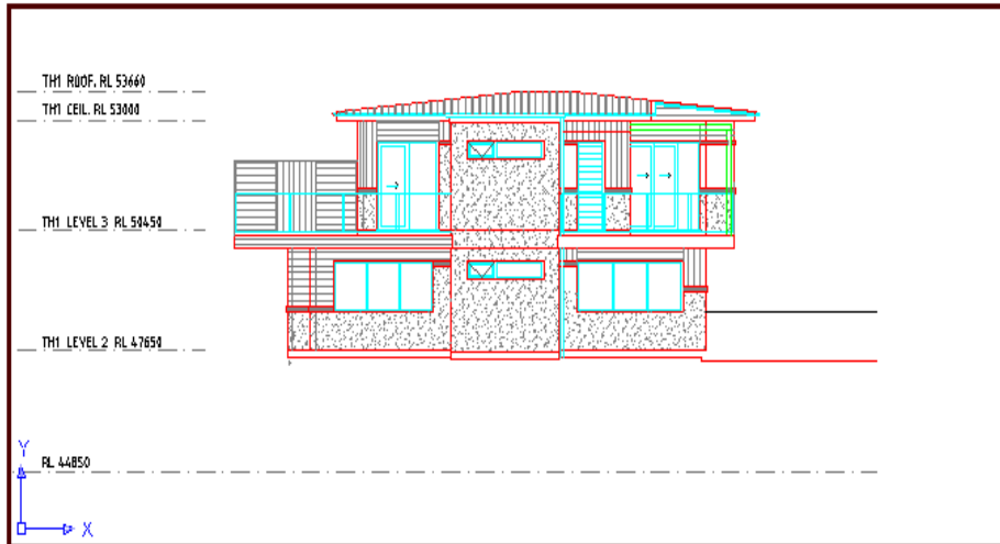
EAST ELEVATION
